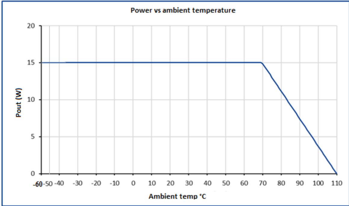
The graph is given for a 15 W model and an efficiency of 88%.
