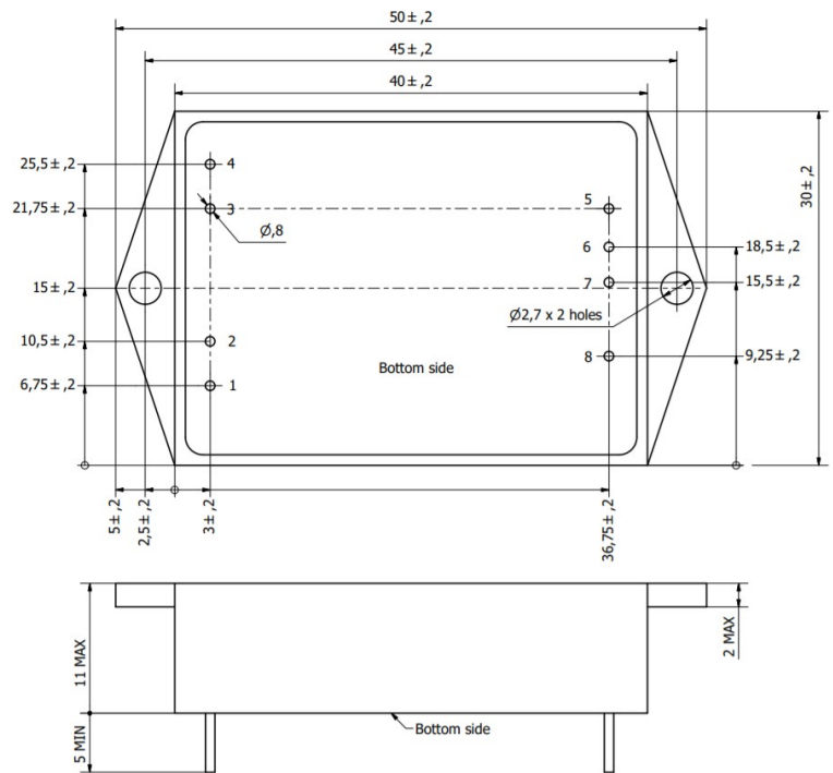
Dual channel
